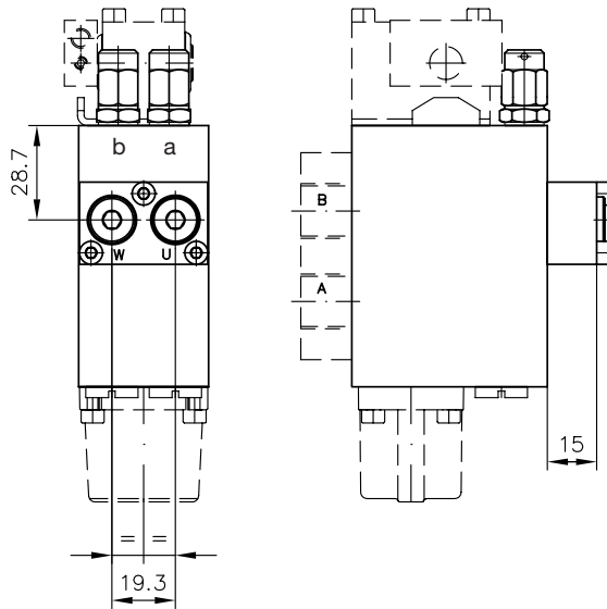
Type A...B...S 1...
