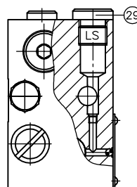
Type PSL.../D-2
