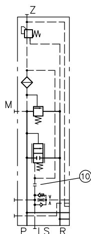
Type PSV...S/D...-2
