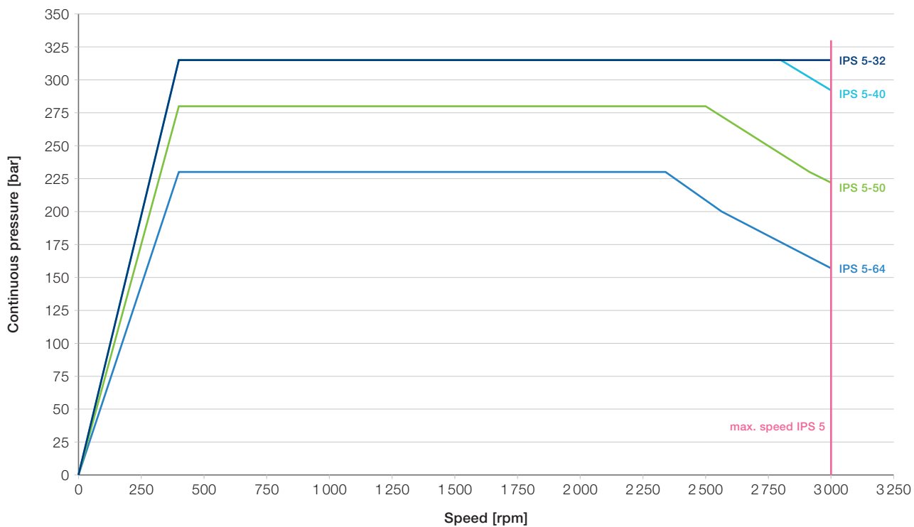
Diagram IPS 5 – Continuous pressure depending on the speed
